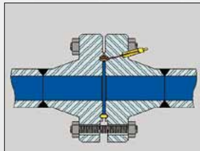
R & RX ring KaMOS® standard (Indicator/test connection horizontal fitted to the flange)
