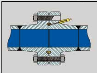
BX ring KaMOS® standard (Indicator/test connection horizontale fitted to the flange)
