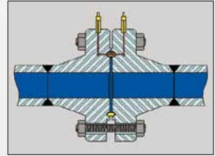
R & RX ring KaMOS® standard (Indicators/test connection in flange)
