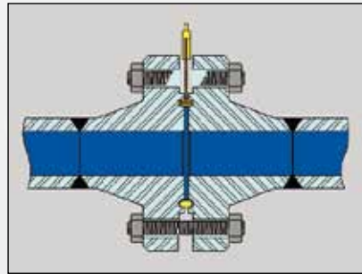
R & RX ring KaMOS® standard (Indicator/test connection in ring)
