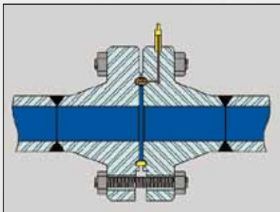
R & RX ring KaMOS® standard (Indicator/test connection fitted to the flange)
