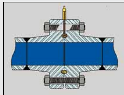
BX ring KaMOS® standard (Indicator/test connection in ring)
