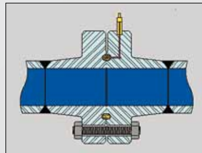
BX ring KaMOS® standard (Indicator/test connection fitted to the flange)
