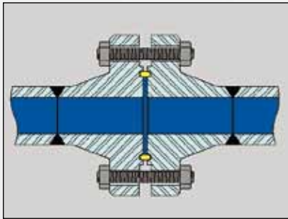
R & RX ring standard
