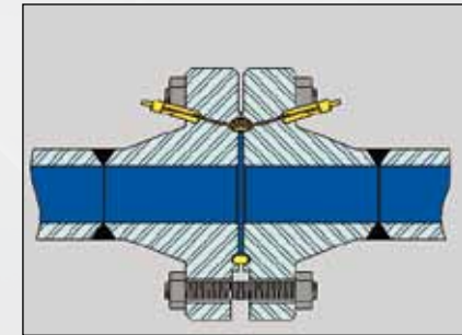
R & RX ring KaMOS® standard (Indicators/test connection horizontal fitted to the flange)
